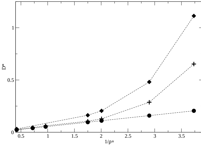
Figure 4.7: The dimensionless dispersion coefficient D^* (diamonds) as a function of inverse dimensionless density \rho^* . Also plotted are the theoretical values of the dimensionless dispersion coefficient D_{th}^* (circles) and the dispersion coefficient obtained by approximating the Lagrangian velocity correlation function with the scaled Eulerian function D_{Eul}^* (plus). Note that low values of \rho^* correspond to high point densities so this data extends to the spatially dense regime. The curves are drawn as a guide to the eye.
