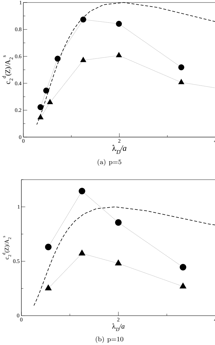
Figure 7.11: Dilute limit of the normalized reduction in the sedimentation velocity of a disk in edgeside motion (spheres) and broadside motion (triangles) compared with the analytic theories valid for a sedimenting sphere of equal surface area (dashed curve) as function of the reduced electric double layer thickness. Disks and spheres have valency Z = 10 . Subfigure (a) refers to a disk with aspect ratio p=5 , and Subfigure (b) to p=10 . Lines joining the simulation points are drawn as guide to the eye.
