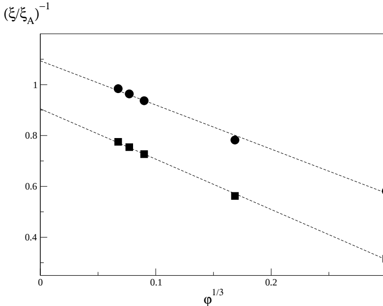
Figure 7.1: Edgeside (circles) and broadside (squares) friction coefficients for a sedimenting neutral disk of aspect ratio p = 5 as function of the array's volume fraction. The friction coefficients are normalized by the friction coefficient of a sphere with radius R = a of the cylinder, i.e. \xi_0 = 6\pi\eta R . The dashed lines are linear fits.
