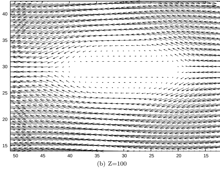
Figure 7.9: 3D flow fields near a charged disk sedimenting along its edge side projected on the plane perpendicular to the disk passing through the center of the disk. The magnitude of the velocities has been conveniently scaled to render them visible.
