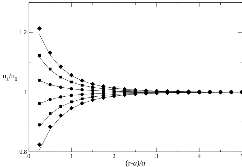
Figure 6.1: Computed n^{\text{PB}}(r)/n_0 (symbols) and approximate n_{\pm}^{\text{LPB}}(r)/n_0 = 1 \mp U^{\text{PB}} (continuous lines) for a surface charge 0.005 (circles), 0.015 (squares), and 0.025 (diamonds). Distance are measured from the surface of the sphere.
