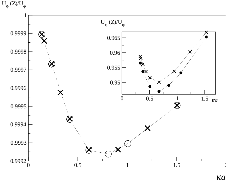
Figure 5.5: Reduced sedimentation velocity of a periodic array of colloids of valency Z = 10 in an electrolyte as a function of \kappa a . The figure shows the results for two different values of the ionic diffusion coefficients. The curve for D_0^{(1)} = 0.95 (circles) has been rescaled to the curve for D_0 = 0.19 (x) according to Eq. (5.31), i.e., U(D) = U(D_0^{(1)}) \times (D_0^{(1)}/D_0) . The superposition of the two curves shows that the scaling is obeyed. In the inset we also show the results for a colloid of valency Z = 100 . However, in this high-charge regime the sedimentation velocity does not scale with the diffusion coefficient in the way predicted by the linearized theory. The dotted lines are a guide to the eye.
