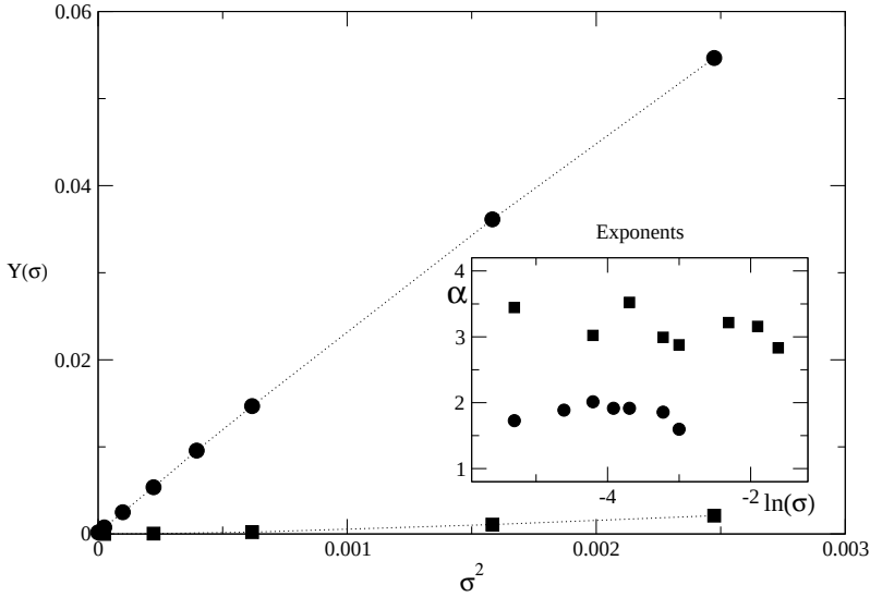
Figure 6.6: \Upsilon(\sigma) as function of the surface charge \sigma , for \kappa a = 1 for a system with added salt (circles) and for a no-added salt one (squares). The dotted lines are guide to the eye.
